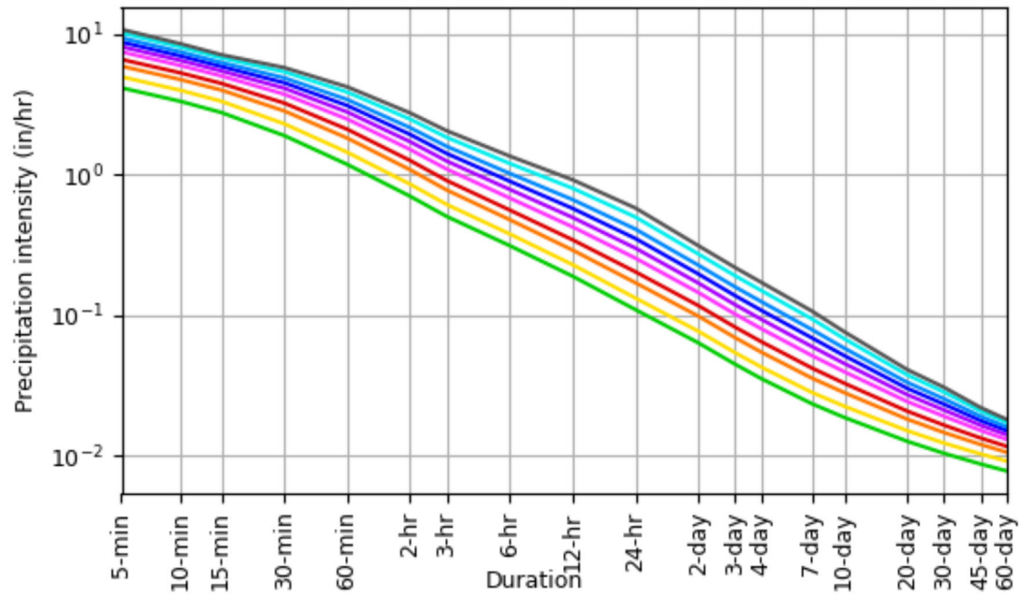
PDS-based intensity-duration-frequency (IDF) curves Latitude: 39.0431°, Longitude: -77.0532°
